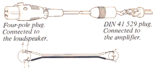
Fig. 7 LOUDSPEAKER LEAD.
